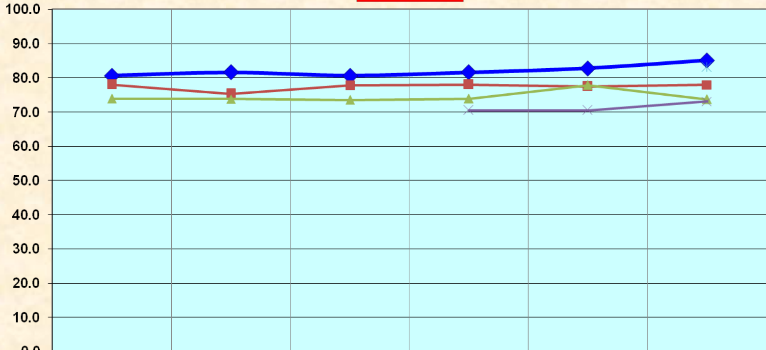
Average Score
